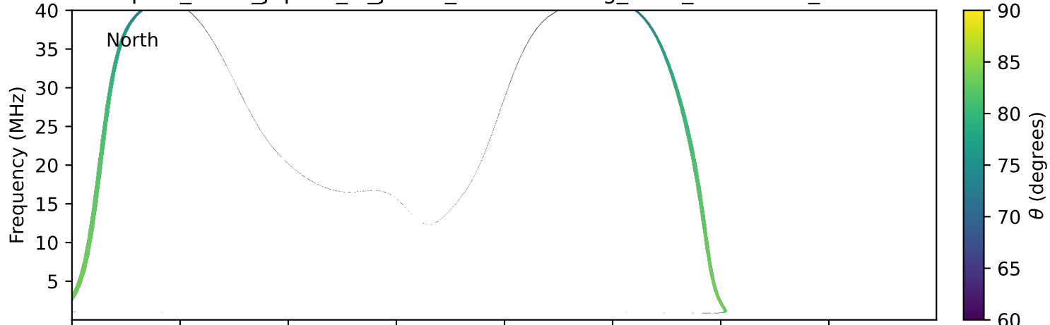
expres_earth_jupiter_io_jrm33_lossc-wid1deg_3kev_20280818_v11.cdf
