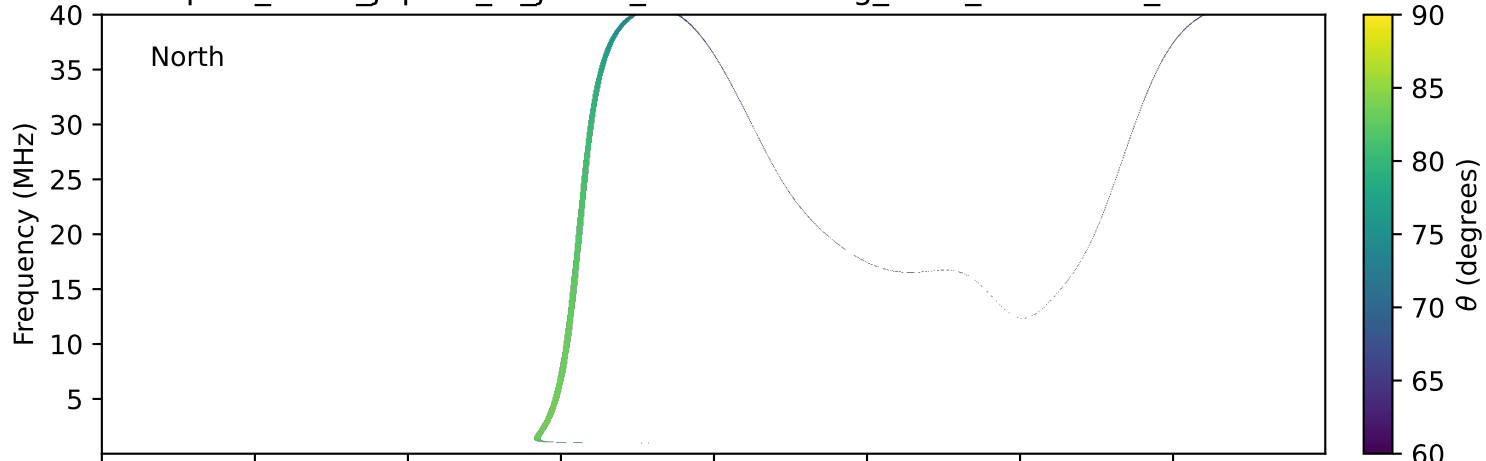
expres_earth_jupiter_io_jrm33_lossc-wid1deg_3kev_20280816_v11.cdf
