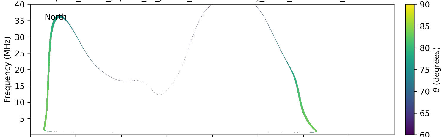
expres_earth_jupiter_io_jrm33_lossc-wid1deg_3kev_20280811_v11.cdf
