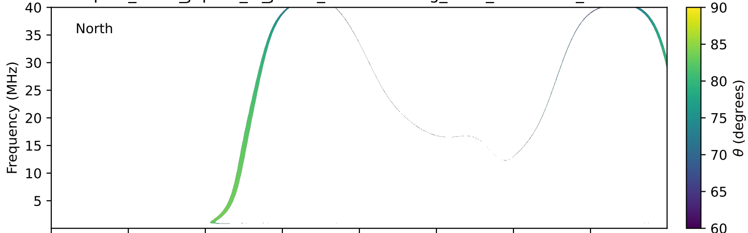
expres_earth_jupiter_io_jrm33_lossc-wid1deg_3kev_20280809_v11.cdf
