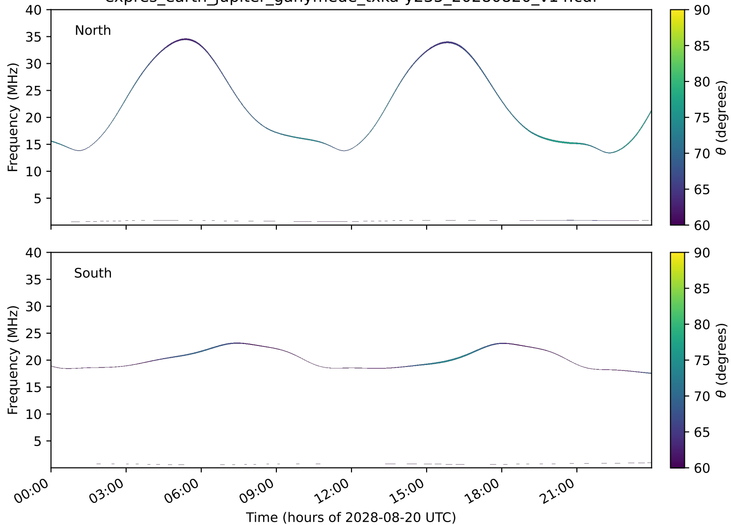
expres_earth_jupiter_ganymede_txka-y235_20280820_v14.cdf
