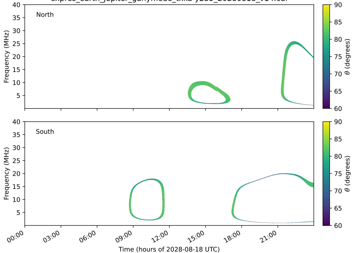
expres_earth_jupiter_ganymede_txka-y235_20280818_v14.cdf
