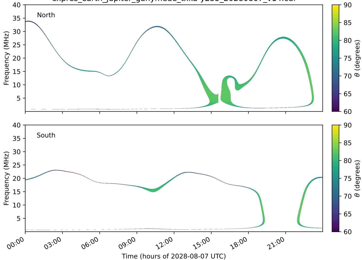
expres_earth_jupiter_ganymede_txka-y235_20280807_v14.cdf
