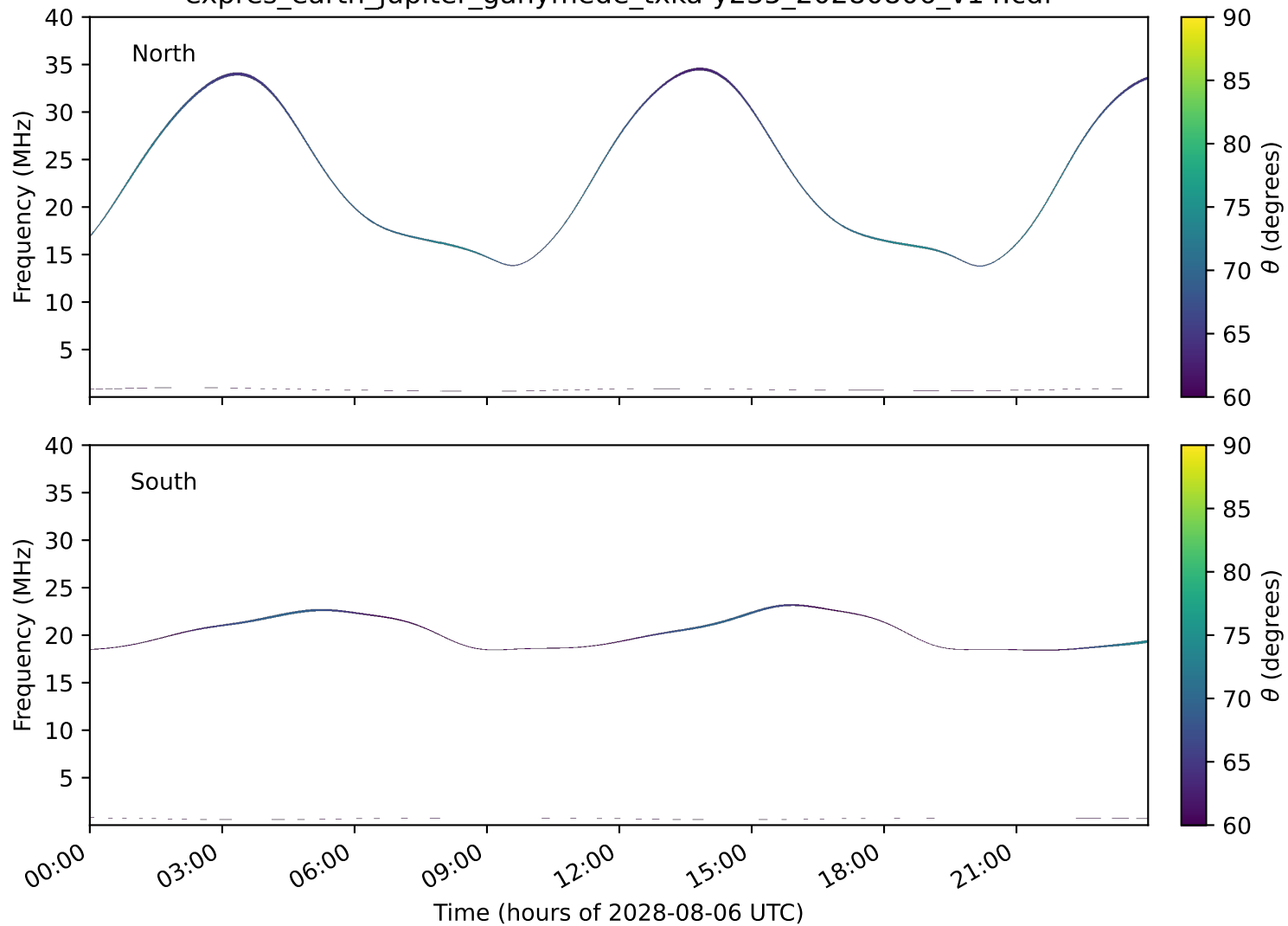
expres_earth_jupiter_ganymede_txka-y235_20280806_v14.cdf
