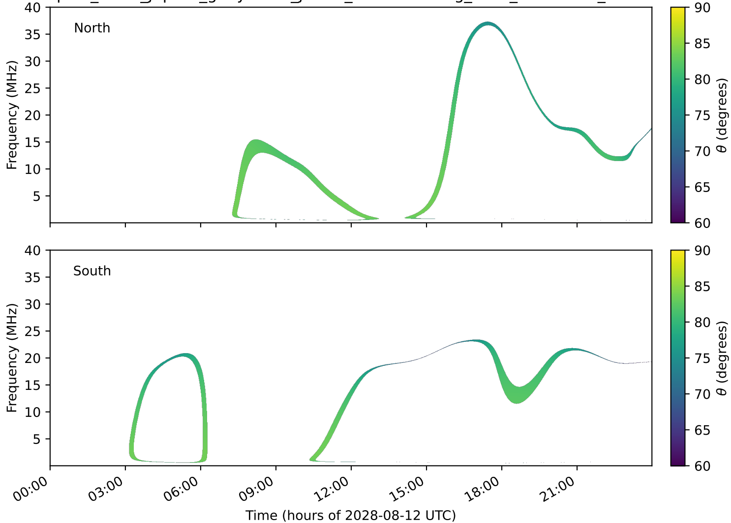
expres_earth_jupiter_ganymede_jrm33_lossc-wid1deg_3kev_20280812_v11.cdf
