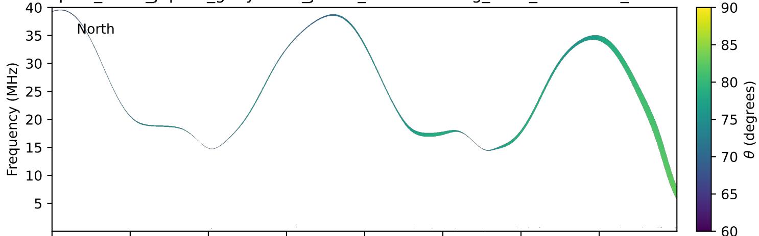
expres_earth_jupiter_ganymede_jrm33_lossc-wid1deg_3kev_20280807_v11.cdf
