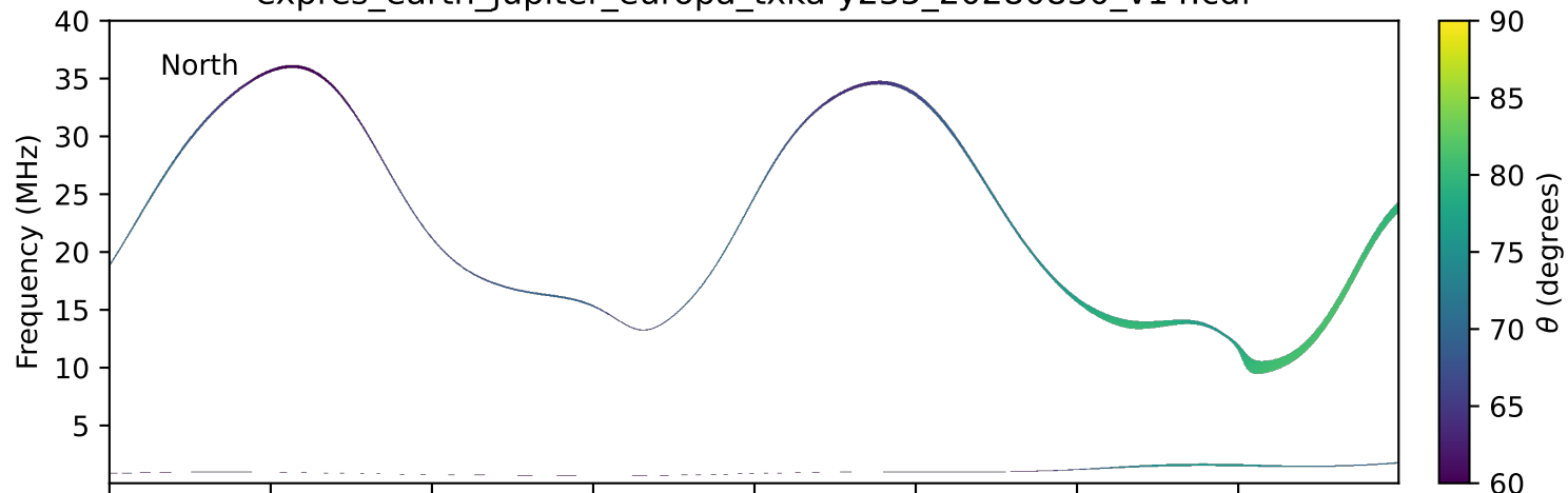
expres_earth_jupiter_europa_txka-y235_20280830_v14.cdf
