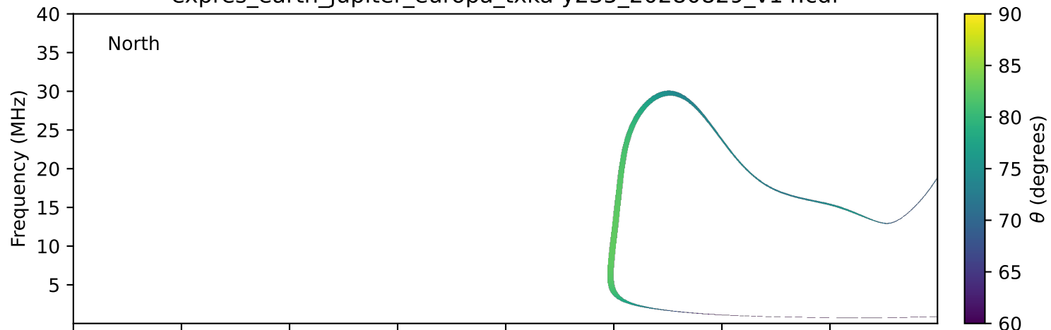
expres_earth_jupiter_europa_txka-y235_20280829_v14.cdf
