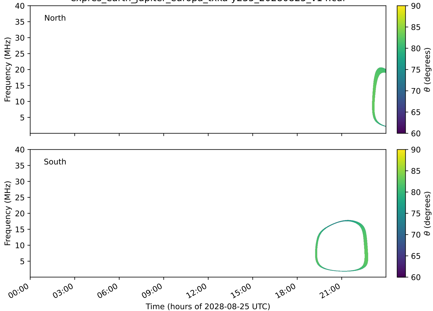
expres_earth_jupiter_europa_txka-y235_20280825_v14.cdf
