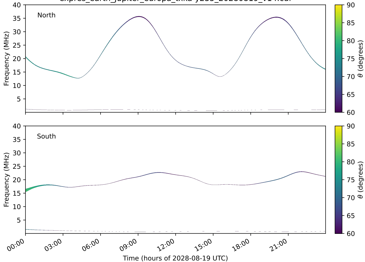
expres_earth_jupiter_europa_txka-y235_20280819_v14.cdf
