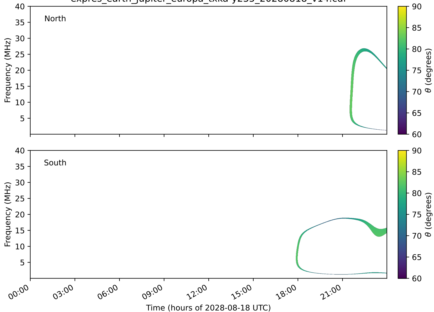
expres_earth_jupiter_europa_txka-y235_20280818_v14.cdf
