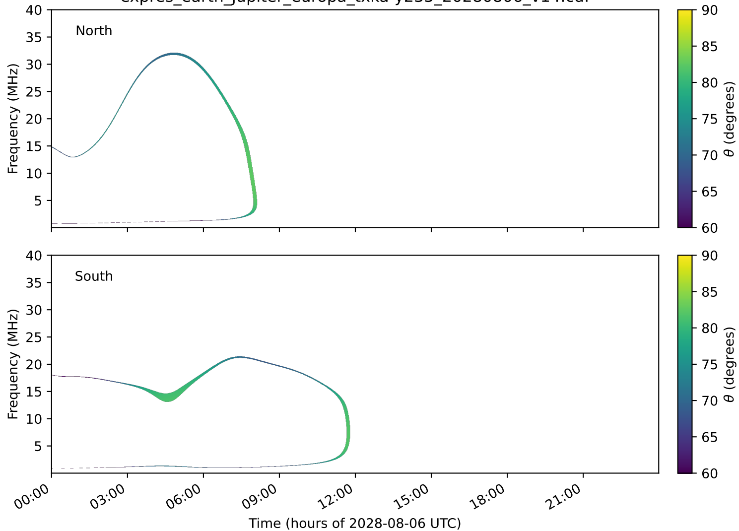
expres_earth_jupiter_europa_txka-y235_20280806_v14.cdf
