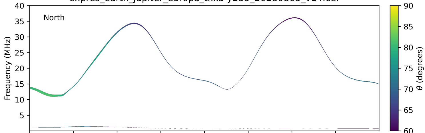
expres_earth_jupiter_europa_txka-y235_20280805_v14.cdf
