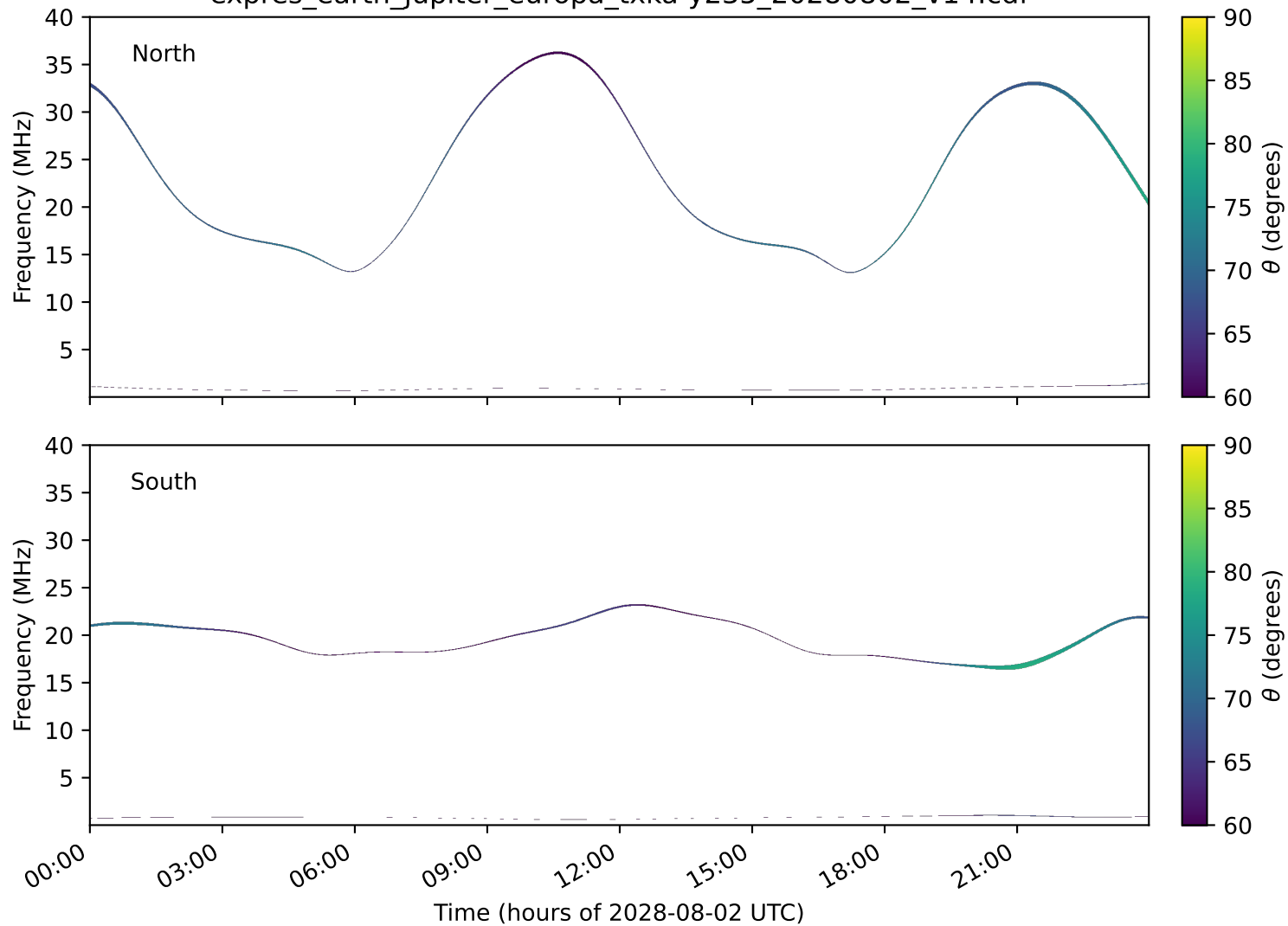
expres_earth_jupiter_europa_txka-y235_20280802_v14.cdf
