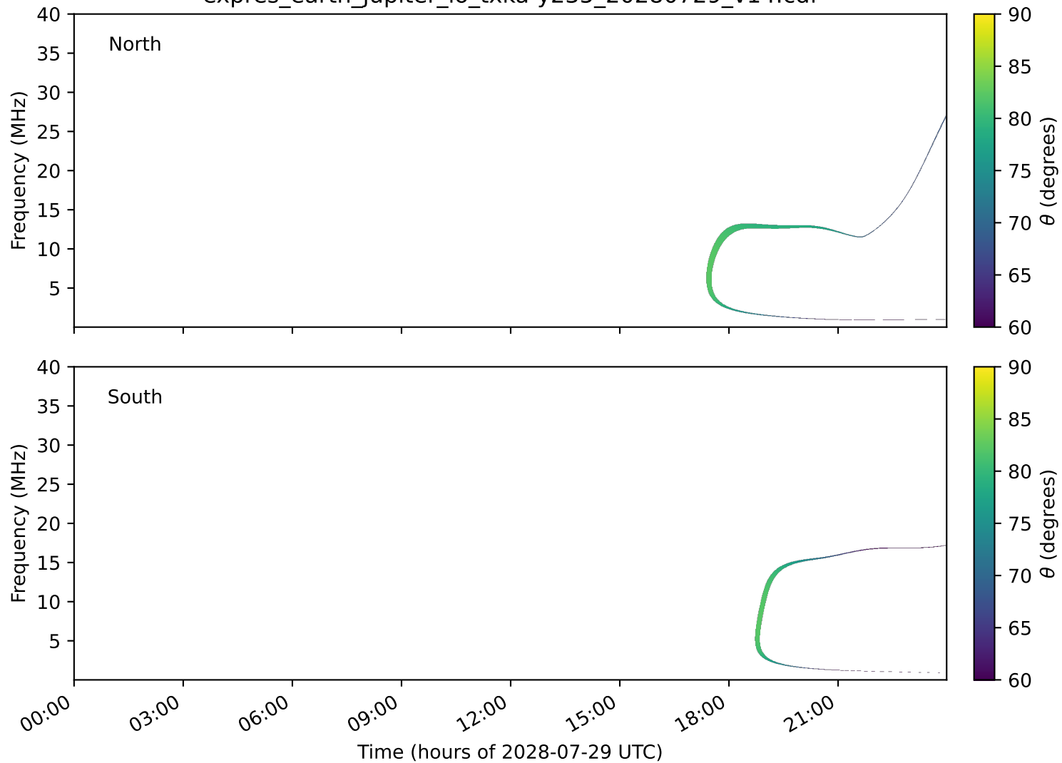
expres_earth_jupiter_io_txka-y235_20280729_v14.cdf
