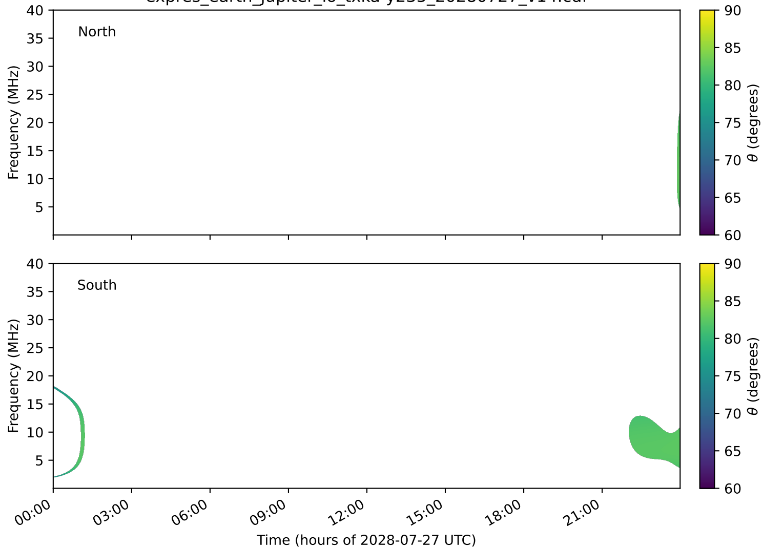
expres_earth_jupiter_io_txka-y235_20280727_v14.cdf
