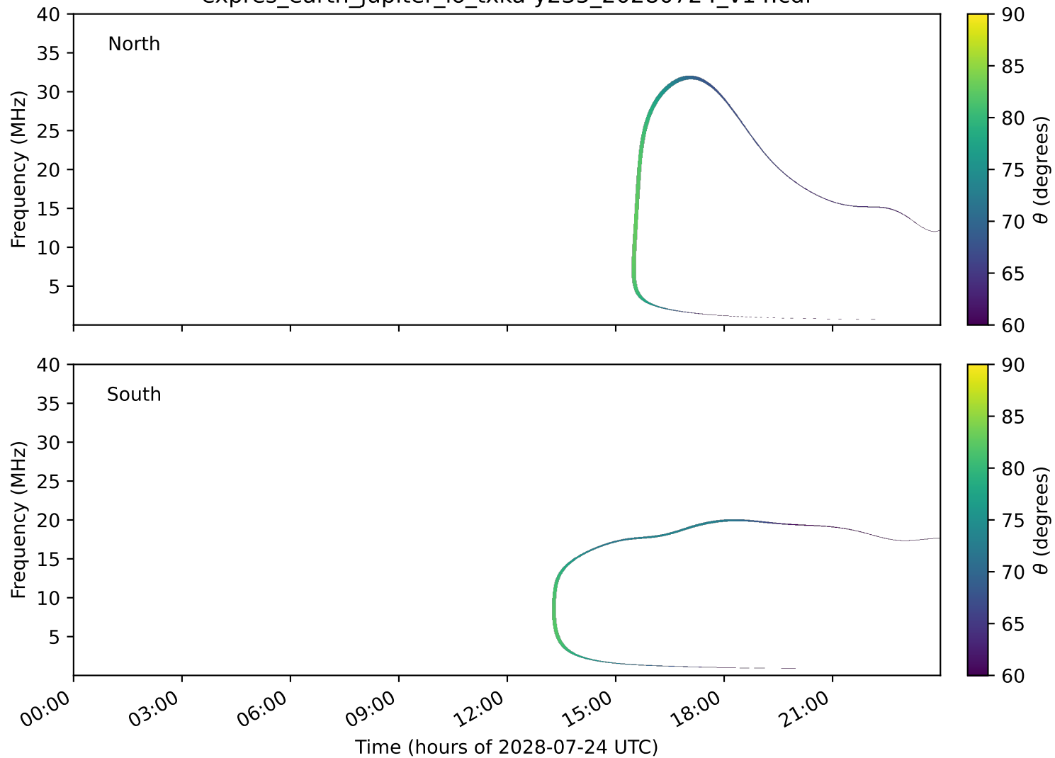
expres_earth_jupiter_io_txka-y235_20280724_v14.cdf
