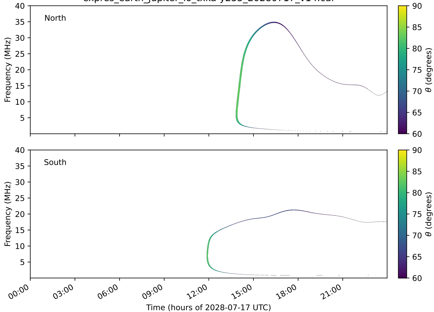
expres_earth_jupiter_io_txka-y235_20280717_v14.cdf
