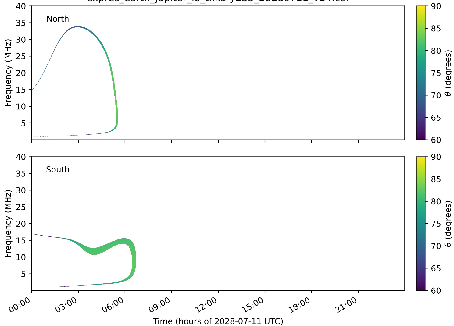
expres_earth_jupiter_io_txka-y235_20280711_v14.cdf
