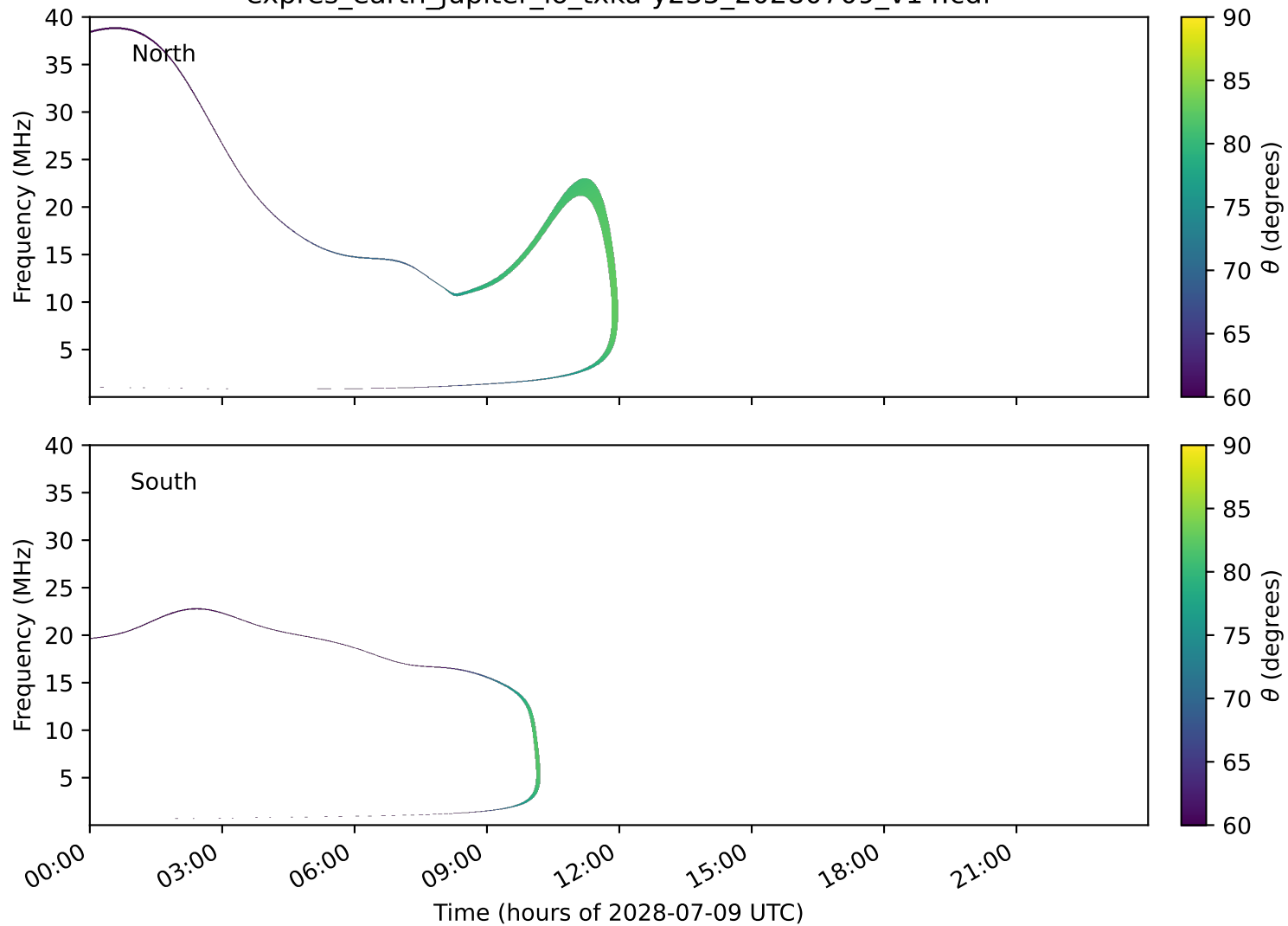
expres_earth_jupiter_io_txka-y235_20280709_v14.cdf
