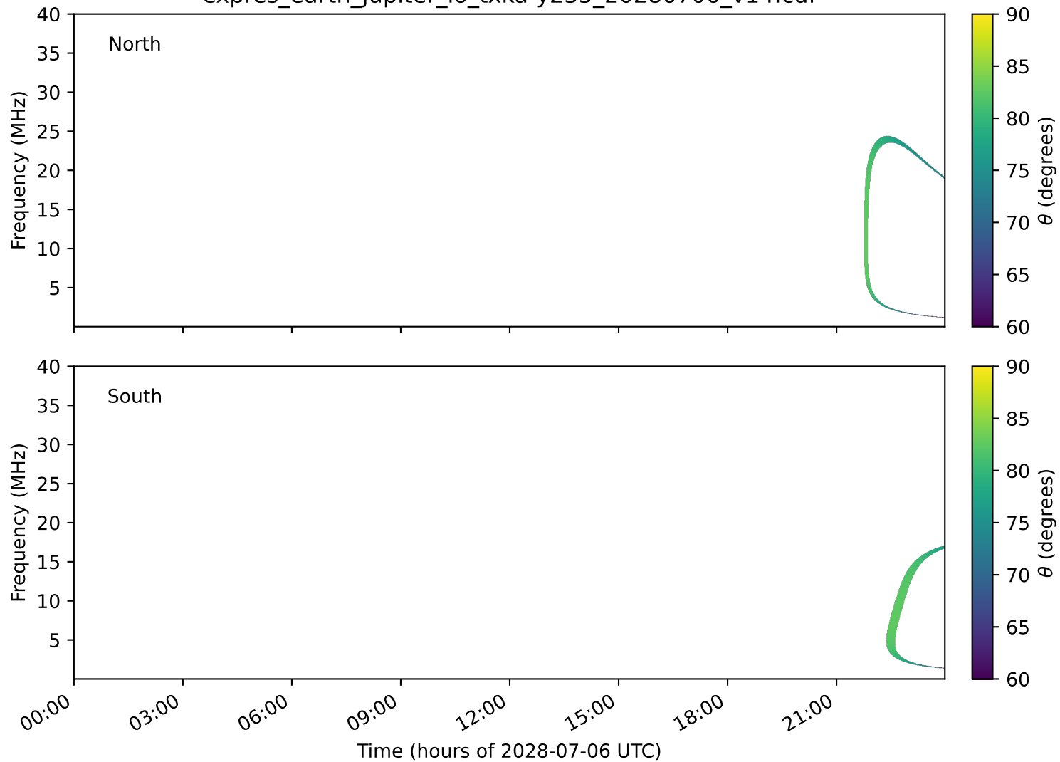
expres_earth_jupiter_io_txka-y235_20280706_v14.cdf
