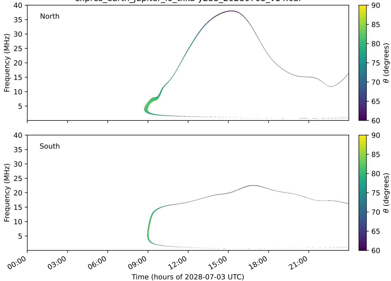
expres_earth_jupiter_io_txka-y235_20280703_v14.cdf
