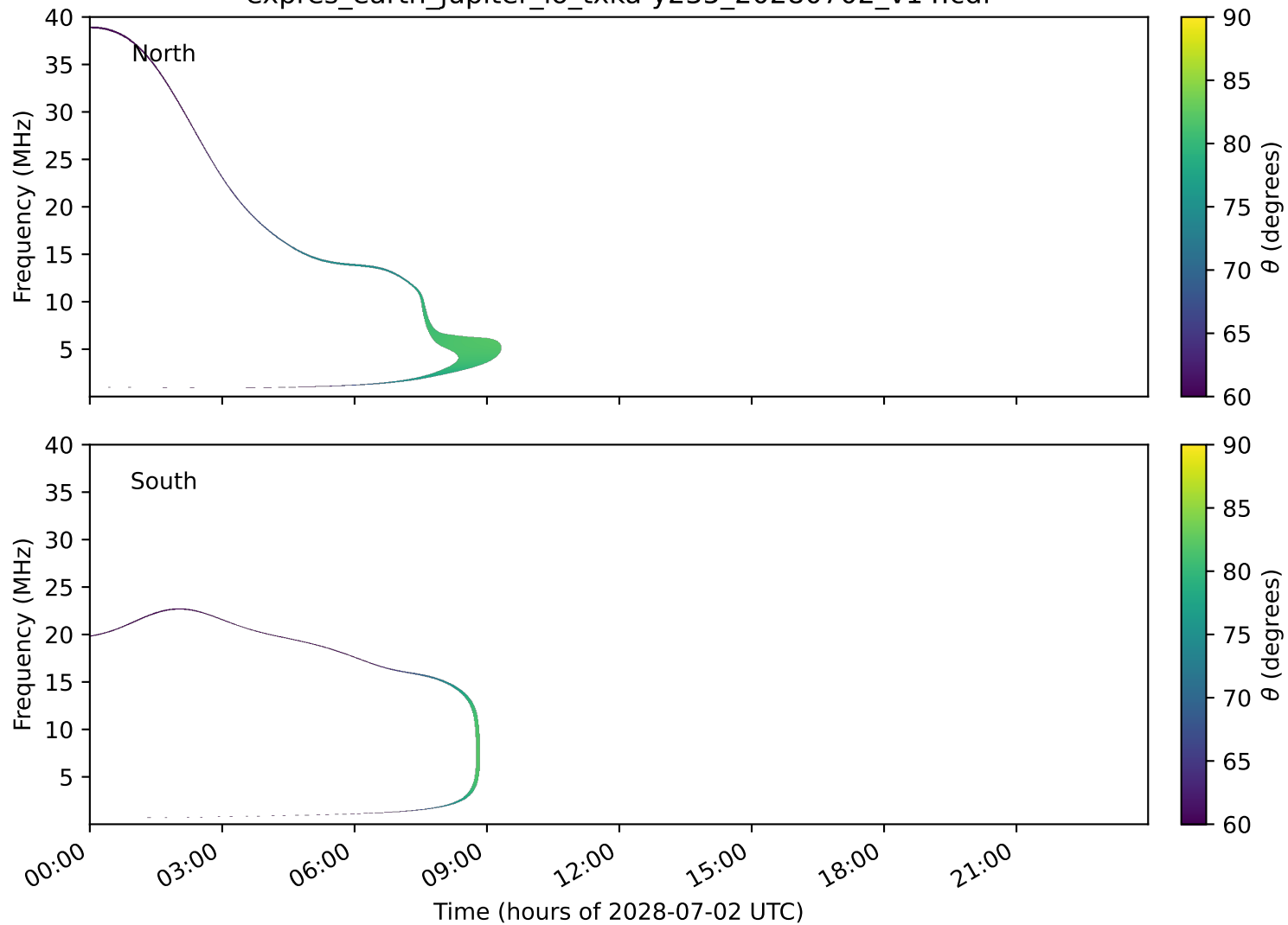
expres_earth_jupiter_io_txka-y235_20280702_v14.cdf
