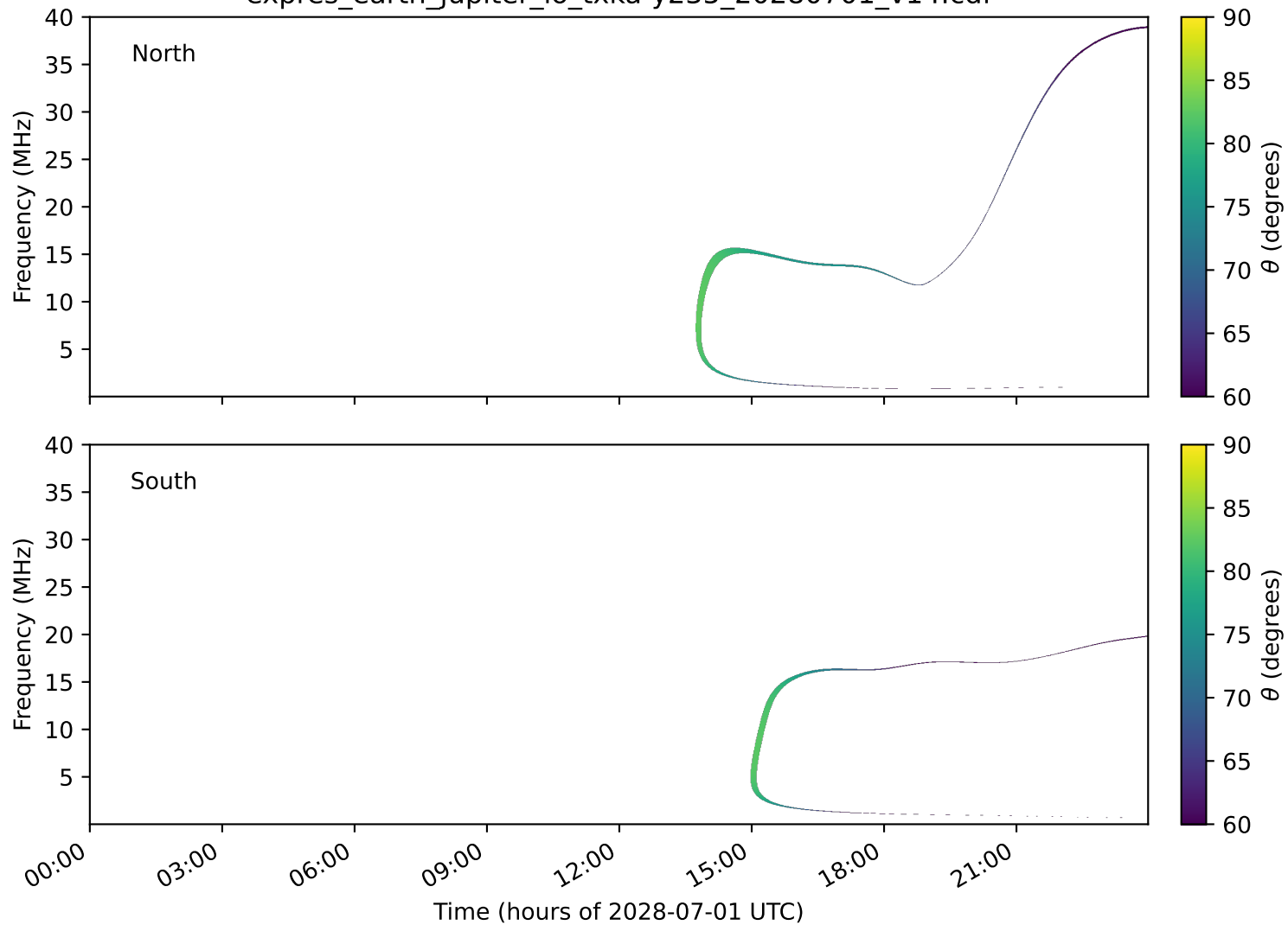
expres_earth_jupiter_io_txka-y235_20280701_v14.cdf
