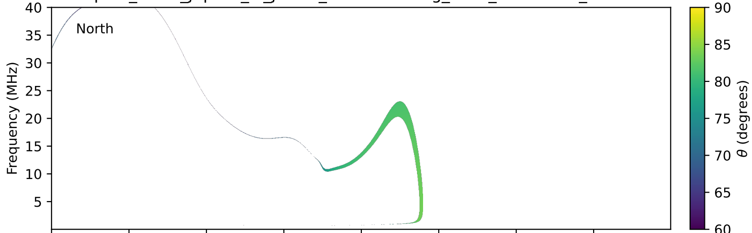
expres_earth_jupiter_io_jrm33_lossc-wid1deg_3kev_20280730_v11.cdf
