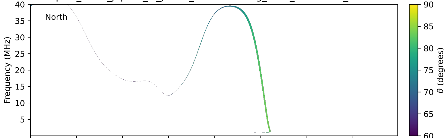
expres_earth_jupiter_io_jrm33_lossc-wid1deg_3kev_20280723_v11.cdf
