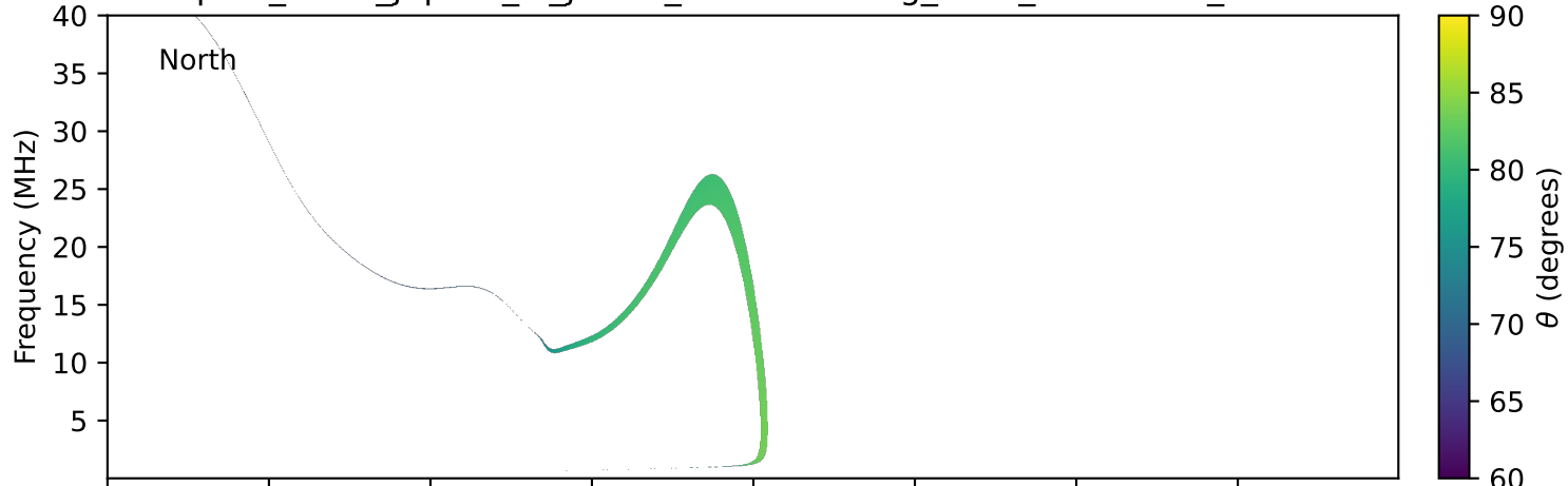
expres_earth_jupiter_io_jrm33_lossc-wid1deg_3kev_20280709_v11.cdf
