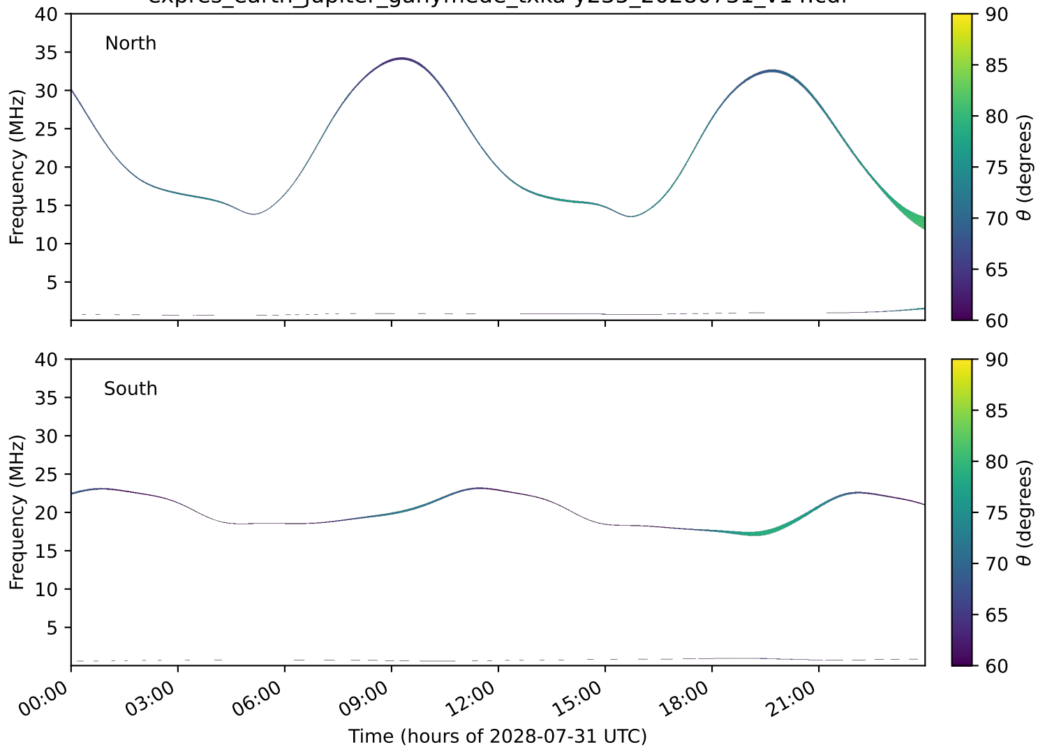
expres_earth_jupiter_ganymede_txka-y235_20280731_v14.cdf
