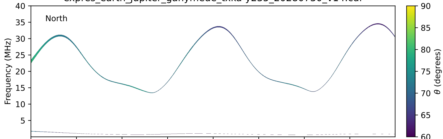
expres_earth_jupiter_ganymede_txka-y235_20280730_v14.cdf
