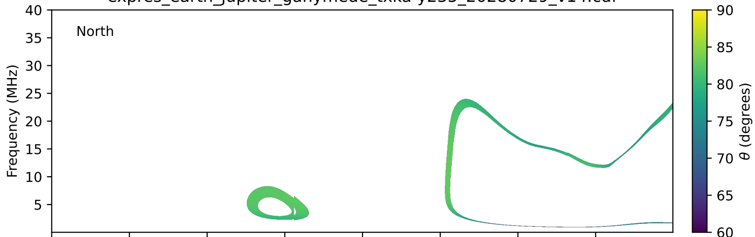
expres_earth_jupiter_ganymede_txka-y235_20280729_v14.cdf
