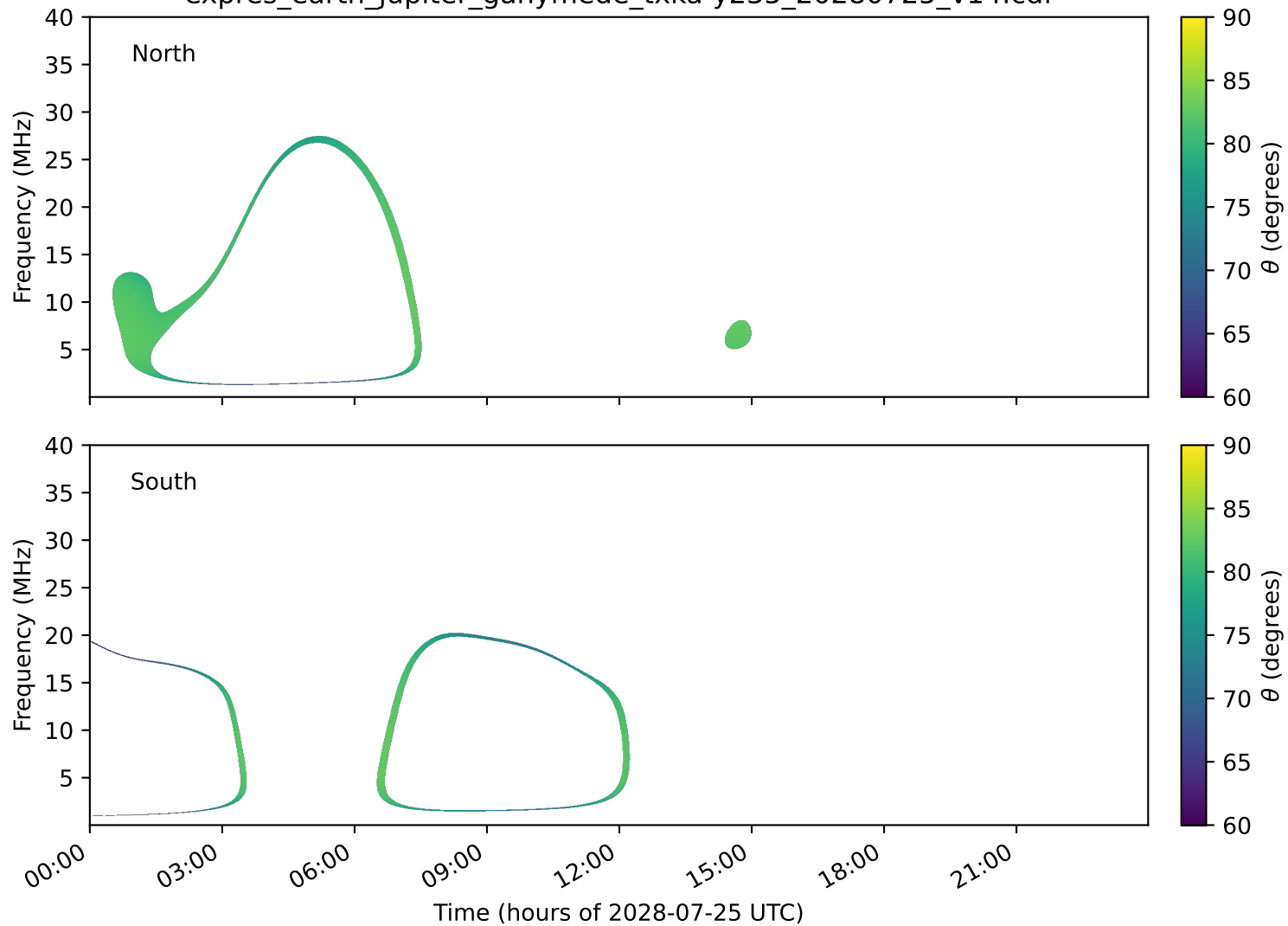
expres_earth_jupiter_ganymede_txka-y235_20280725_v14.cdf
