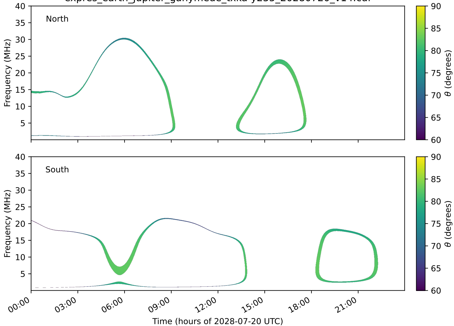
expres_earth_jupiter_ganymede_txka-y235_20280720_v14.cdf
