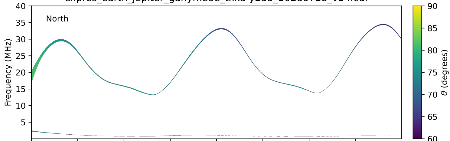
expres_earth_jupiter_ganymede_txka-y235_20280718_v14.cdf
