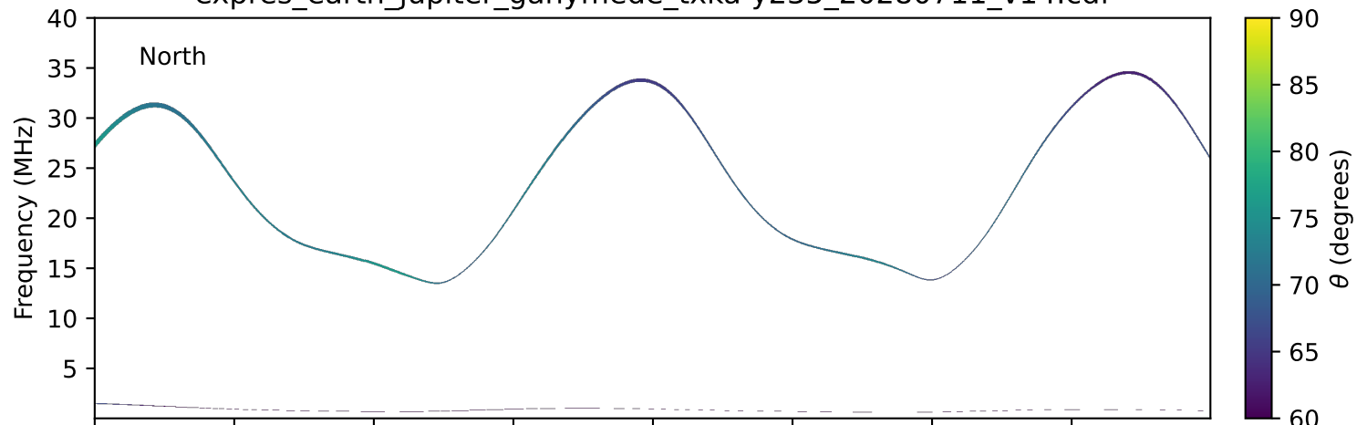
expres_earth_jupiter_ganymede_txka-y235_20280711_v14.cdf
