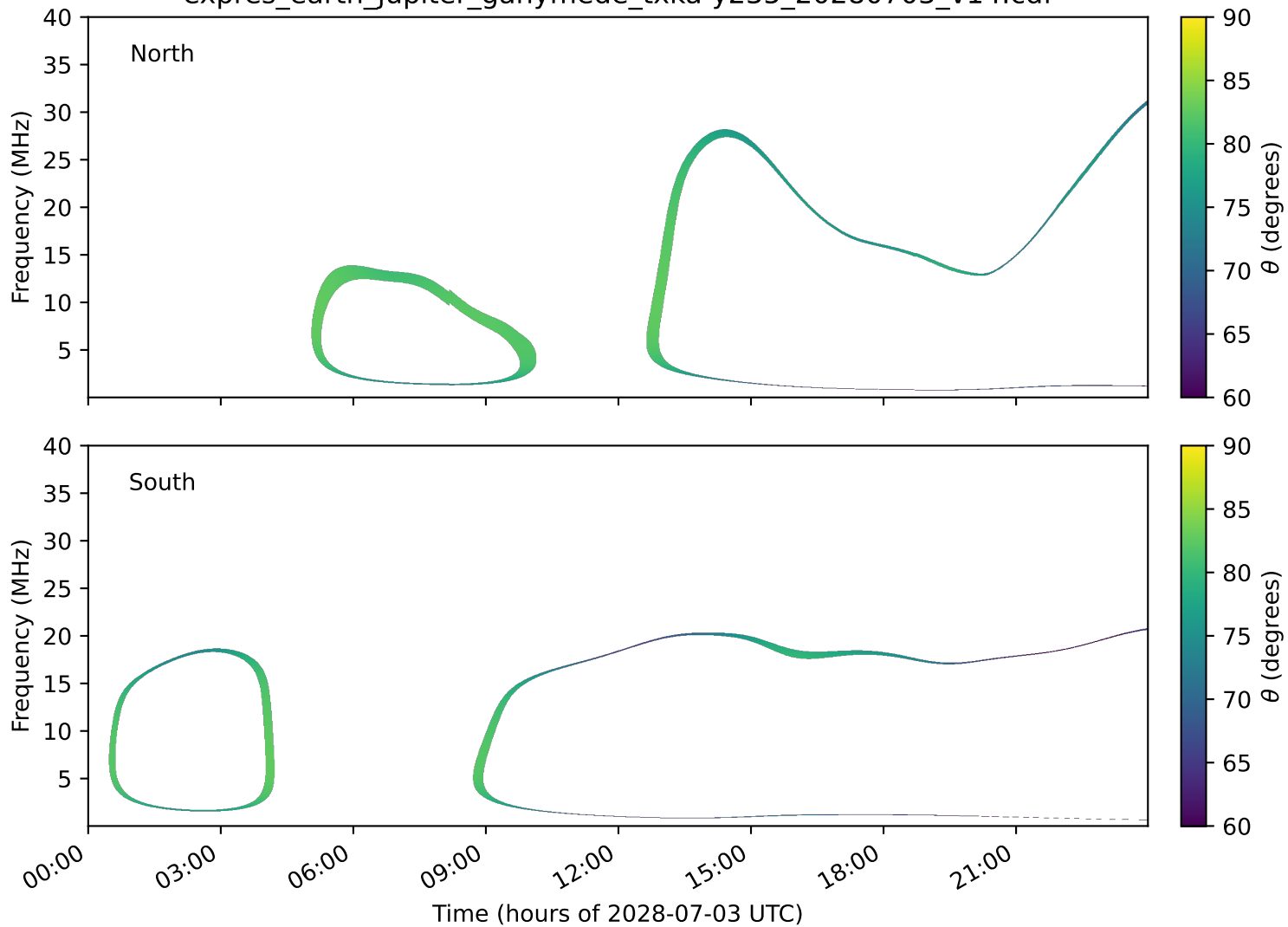
expres_earth_jupiter_ganymede_txka-y235_20280703_v14.cdf
