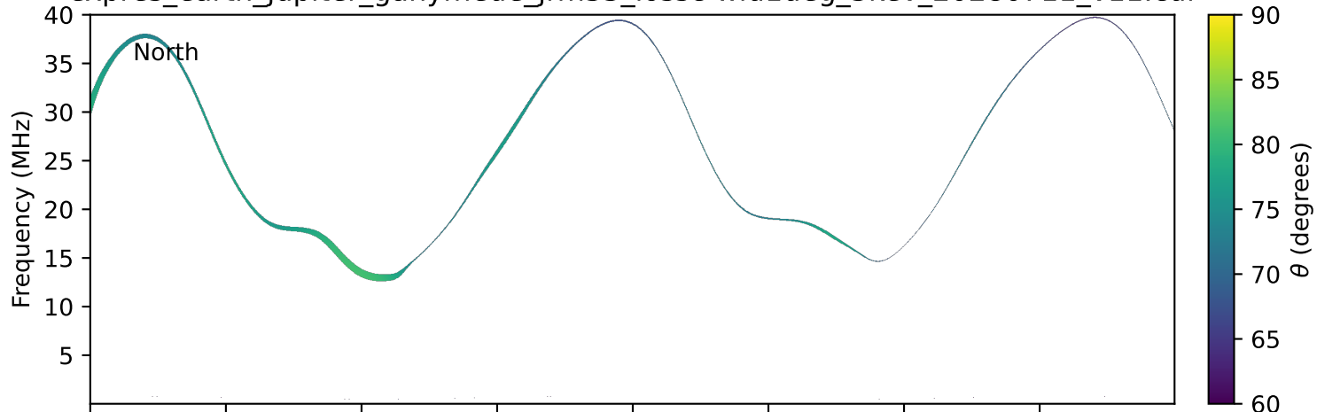
expres_earth_jupiter_ganymede_jrm33_lossc-wid1deg_3kev_20280711_v11.cdf
