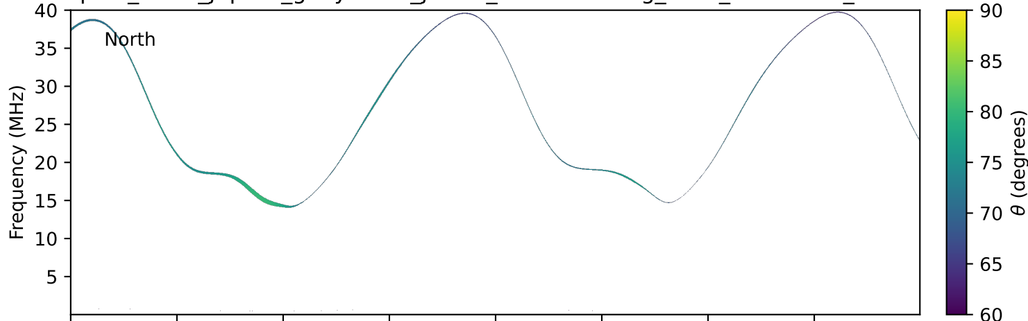
expres_earth_jupiter_ganymede_jrm33_lossc-wid1deg_3kev_20280704_v11.cdf
