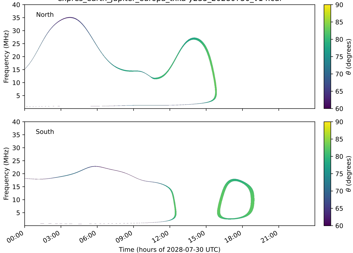
expres_earth_jupiter_europa_txka-y235_20280730_v14.cdf
