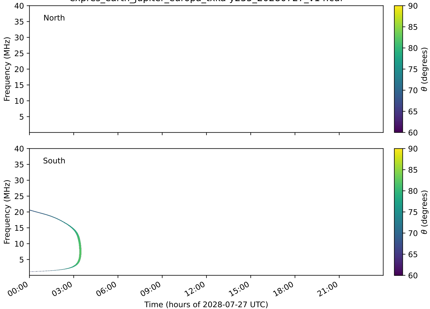
expres_earth_jupiter_europa_txka-y235_20280727_v14.cdf
