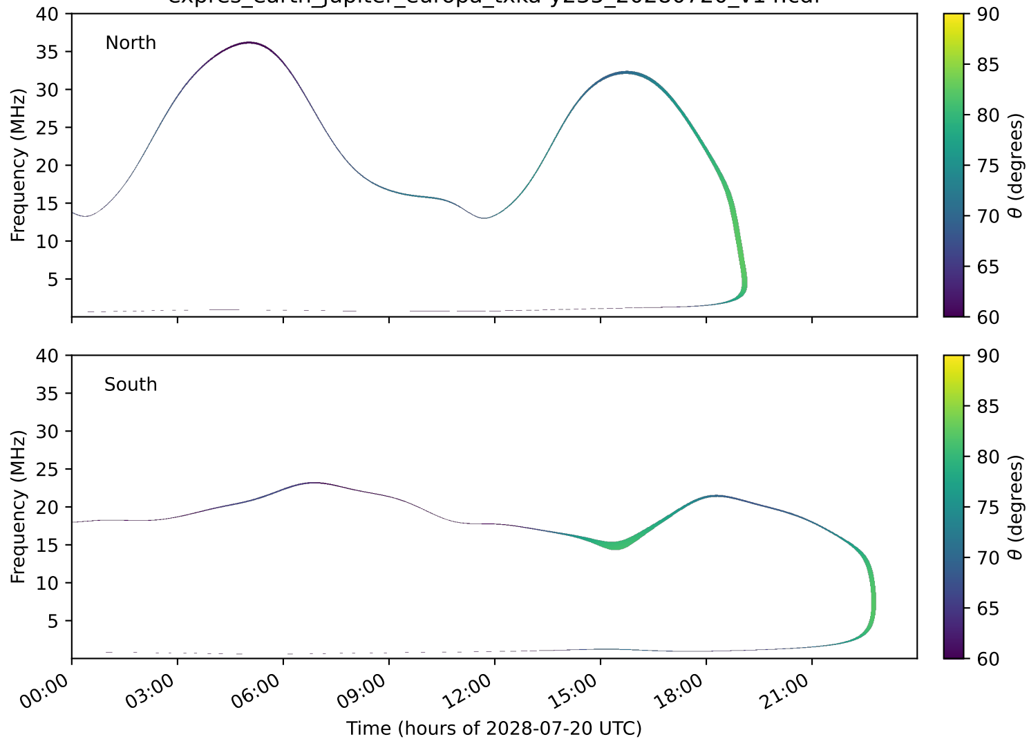
expres_earth_jupiter_europa_txka-y235_20280720_v14.cdf
