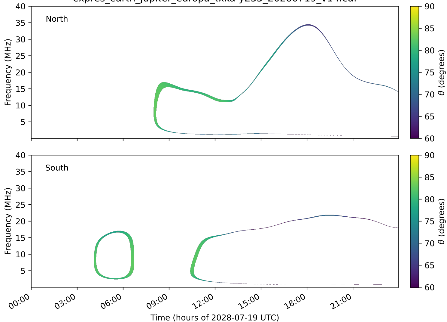
expres_earth_jupiter_europa_txka-y235_20280719_v14.cdf
