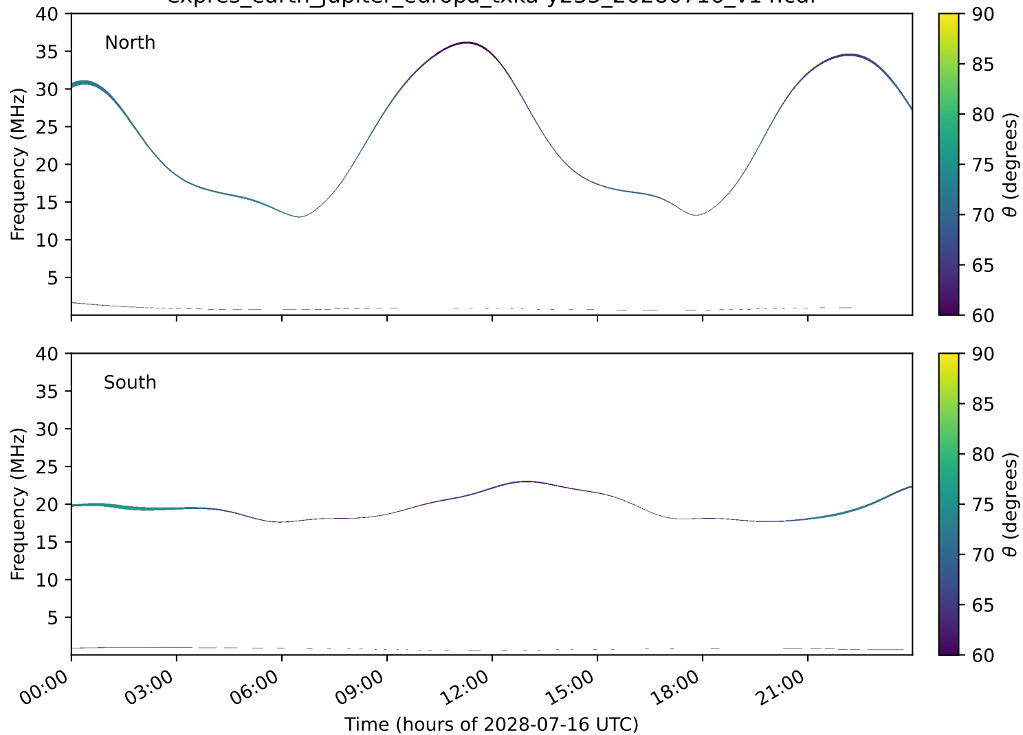
expres_earth_jupiter_europa_txka-y235_20280716_v14.cdf
