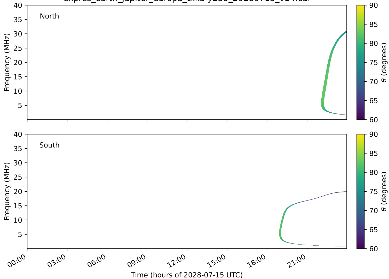
expres_earth_jupiter_europa_txka-y235_20280715_v14.cdf
