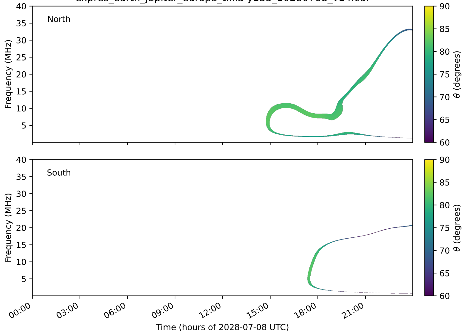
expres_earth_jupiter_europa_txka-y235_20280708_v14.cdf
