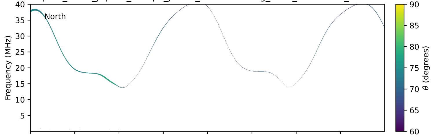
expres_earth_jupiter_europa_jrm33_lossc-wid1deg_3kev_20280716_v11.cdf
