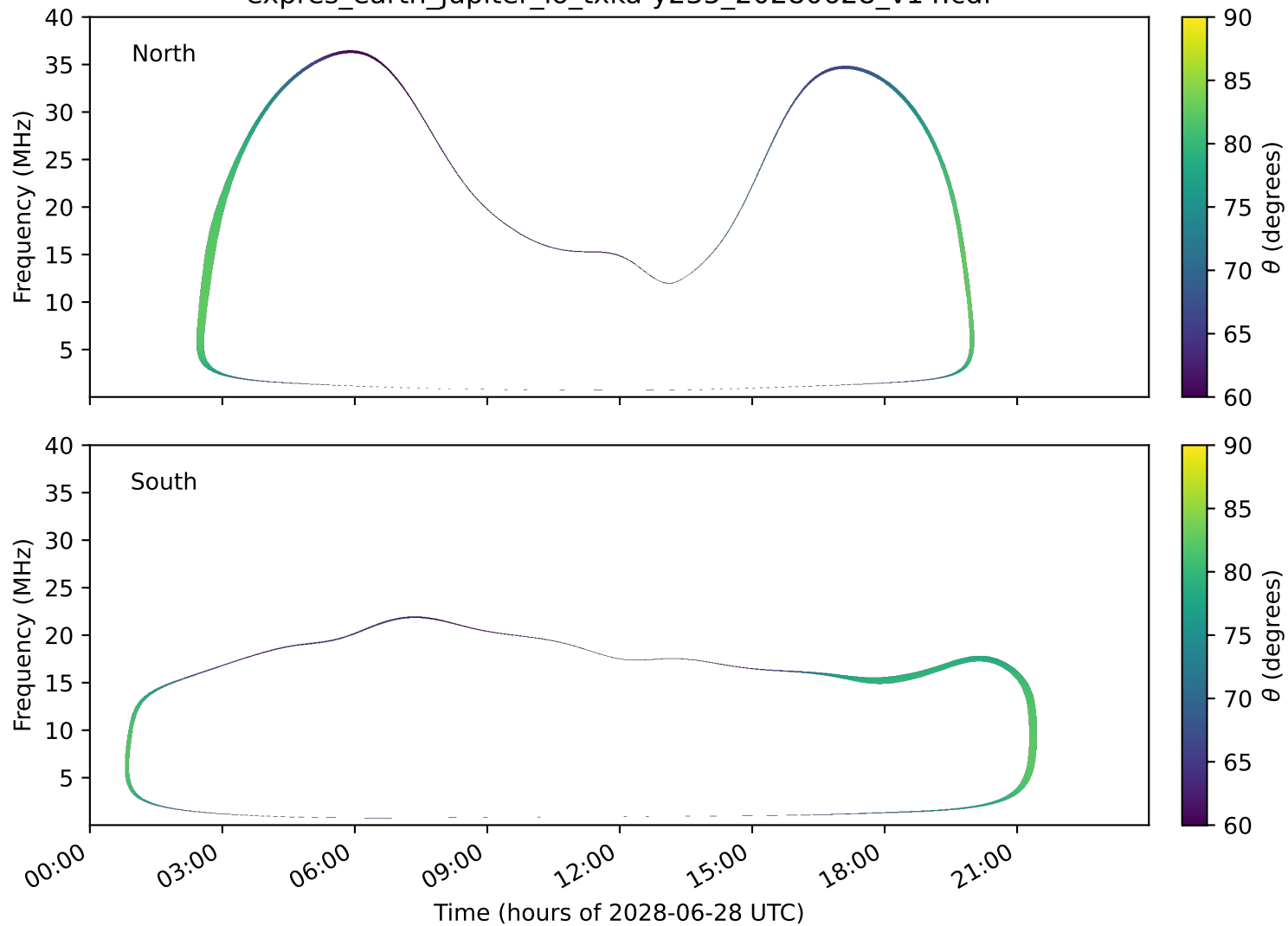
expres_earth_jupiter_io_txka-y235_20280628_v14.cdf
